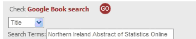
Figure 3: getWebSearch
